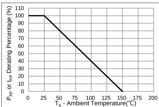
Fig.4 Derating Curve
