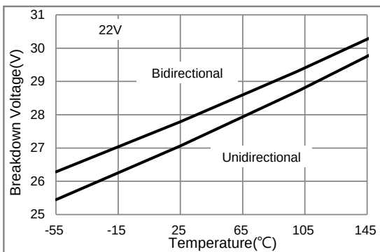
Fig.6 Typical V_{BR} versus Temperature
