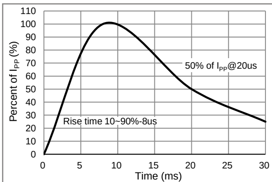
Fig.2 Pulse Waveform
