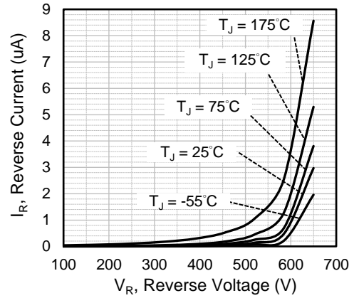
Fig.2 Reverse Characteristics
