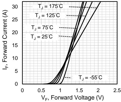
Fig.1 Forward Characteristics
