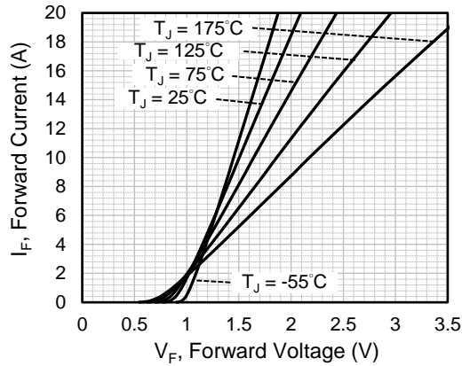
Fig.1 Forward Characteristics
