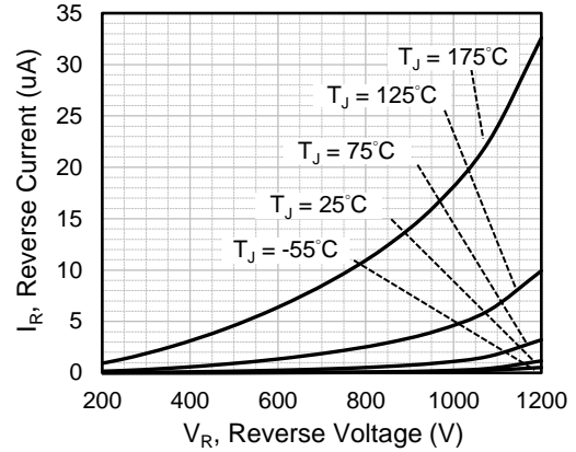
Fig.2 Reverse Characteristics
