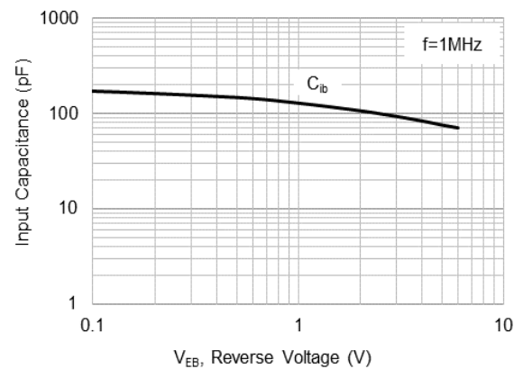
Fig.9 Input Capacitance
