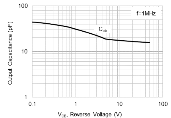
Fig.10 Output Capacitance
