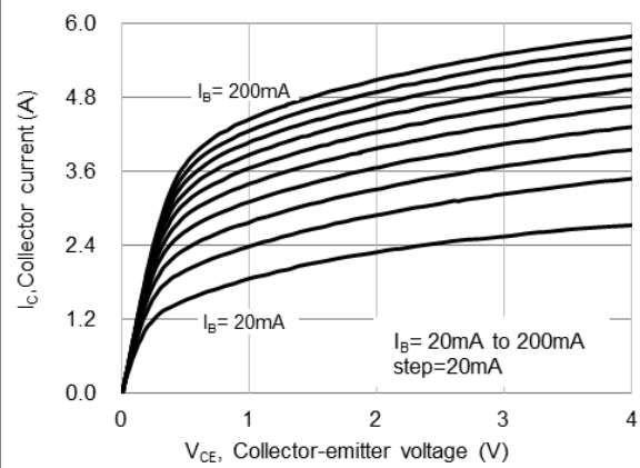
Fig.8 Collector Current
