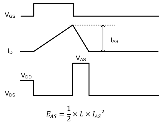
Fig.24 Avalanche Waveform
