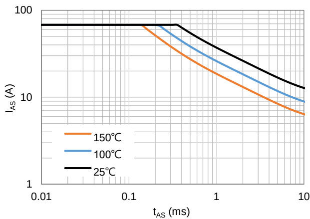
Fig.13 Avalanche characteristics
