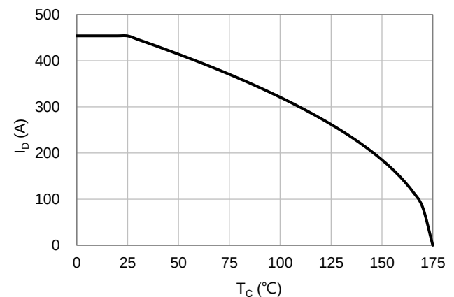
Fig.12 Drain Current vs. Case Temperature
