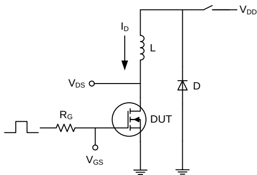
Fig.23 Avalanche Test Circuit
