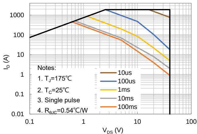
Fig.17 Maximum Safe Operating Area
