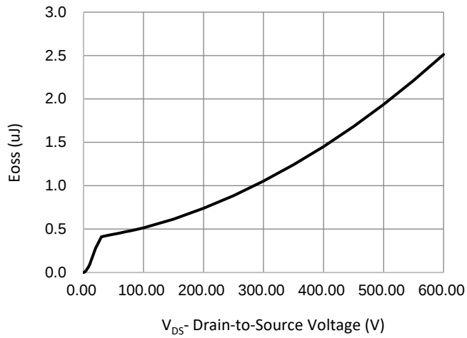
Fig.13 Typ. Coss Stored Energy
