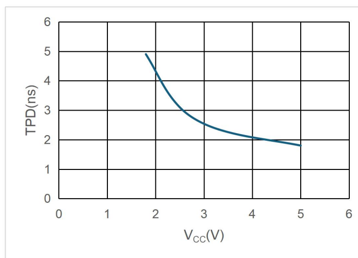
T PD across V CC at 25°C
