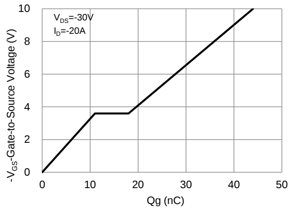
Fig.7 Gate-Charge Characteristics
