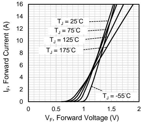
Fig.1 Forward Characteristics
