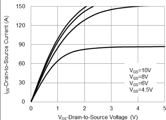
Fig.1 On-Region Characteristics
