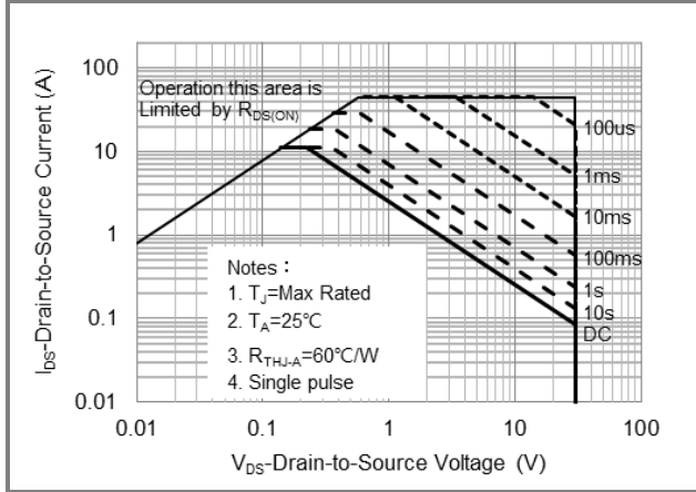
Fig.13 Maximum Safe Operating Area
