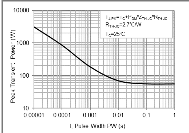
Fig.15 Single Pulse Maximum Power Dissipation
