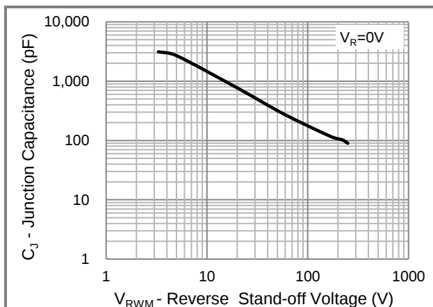
Fig.4 Typical Capacitance
