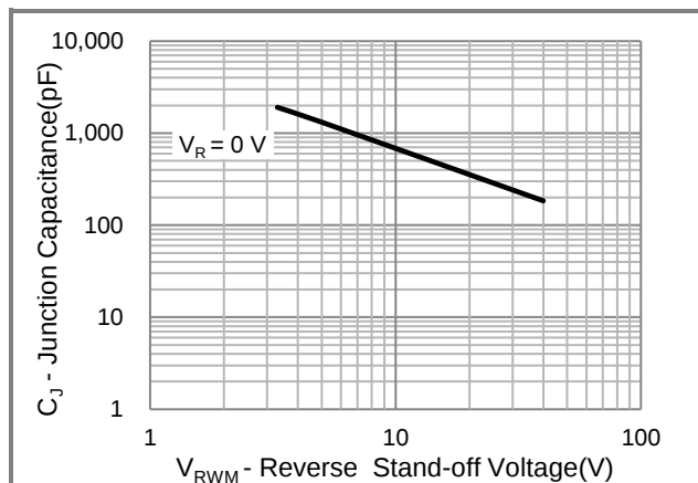
Fig.4 Typical Capacitance
