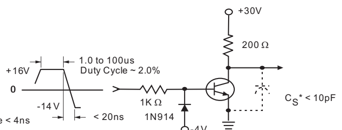
Fig. 2 Turn-Off Time
