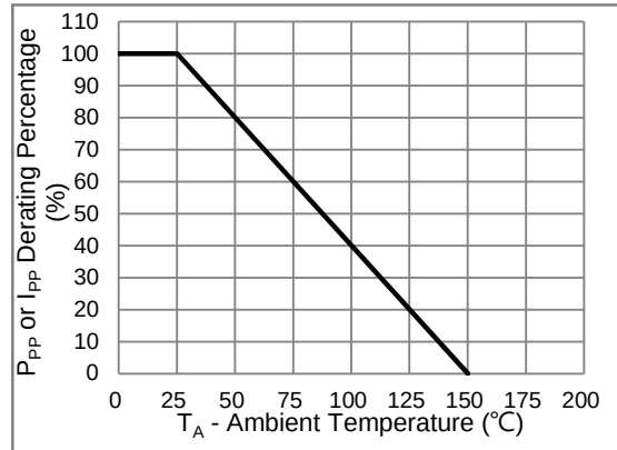
Fig.2 Derating Curve
