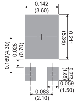
TO-277C
