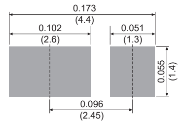
SOD-123HE
