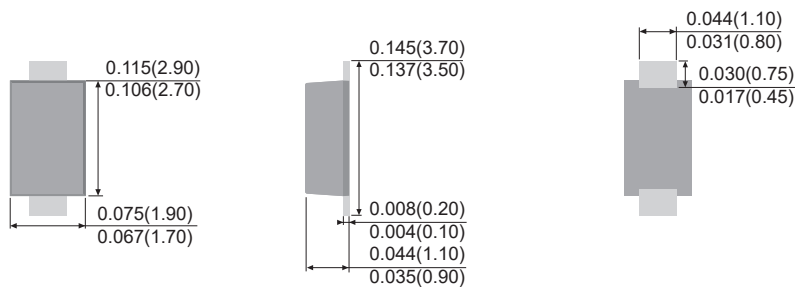
SOD-123FL
