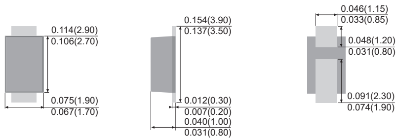
SOD-123FL
